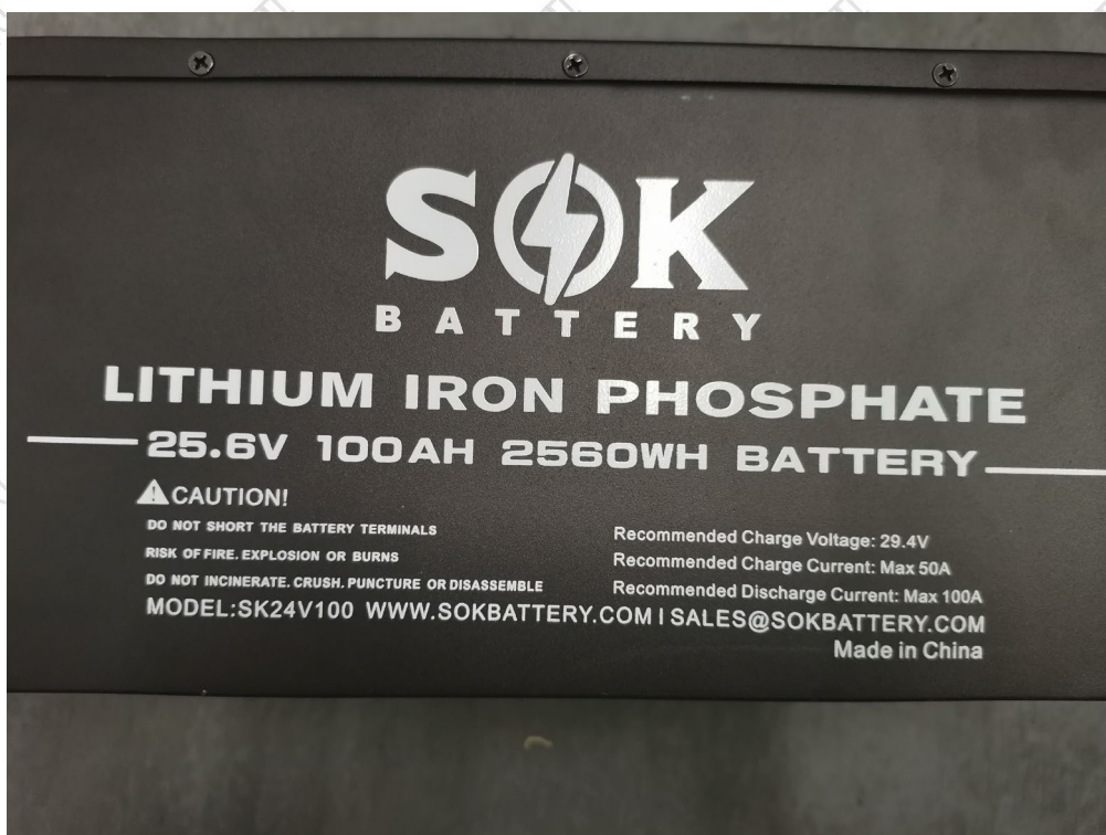
Figure 4 Battery Label
