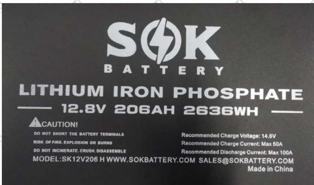
Figure 4 Battery Label
